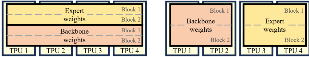
(a) A model-parallel partitioning in which an entire MoDE model is split across all TPUs. (b) An flexible sharding configuration enabled by the MoDE architecture and MPMD.
